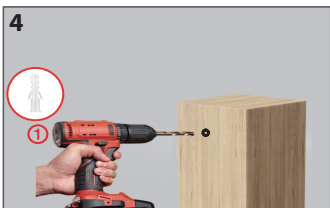
4.Mark and drill holes and hammer the plastic insert into the holes.
